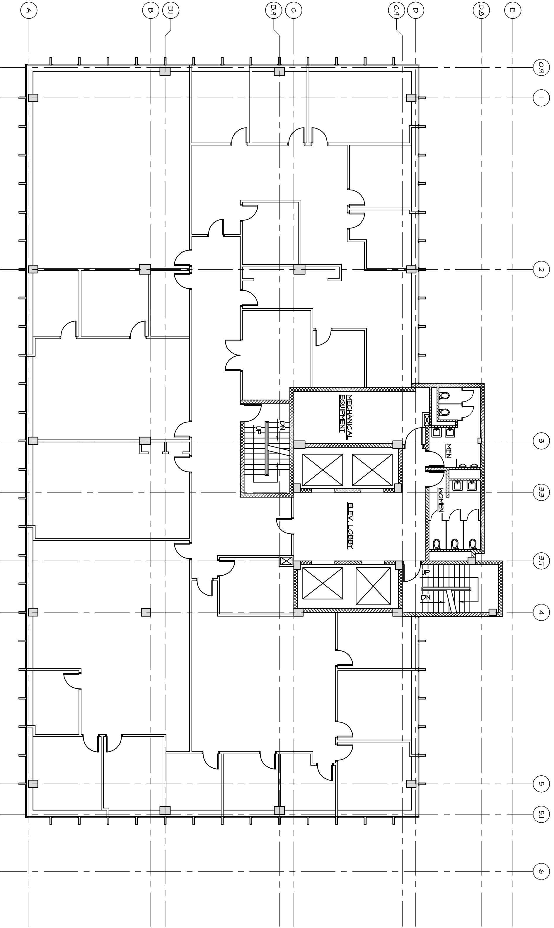
EIGHTH LEVEL FLOOR PLAN
