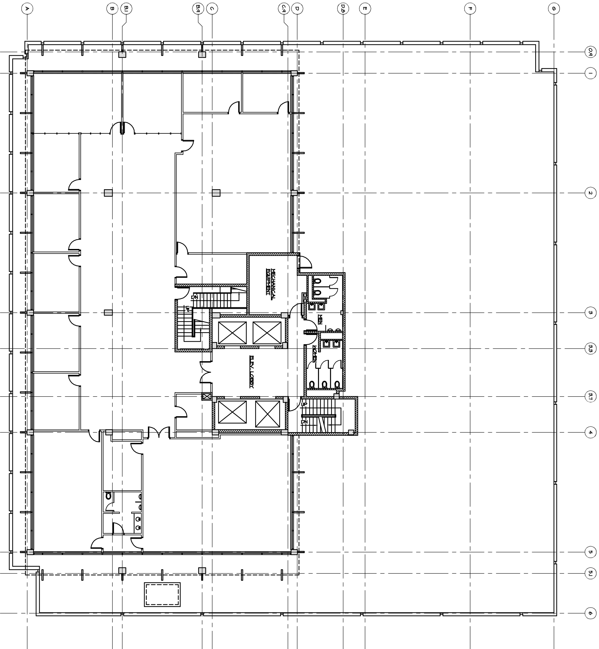
SIXTH FLOOR PLAN - TERRACE LEVEL
