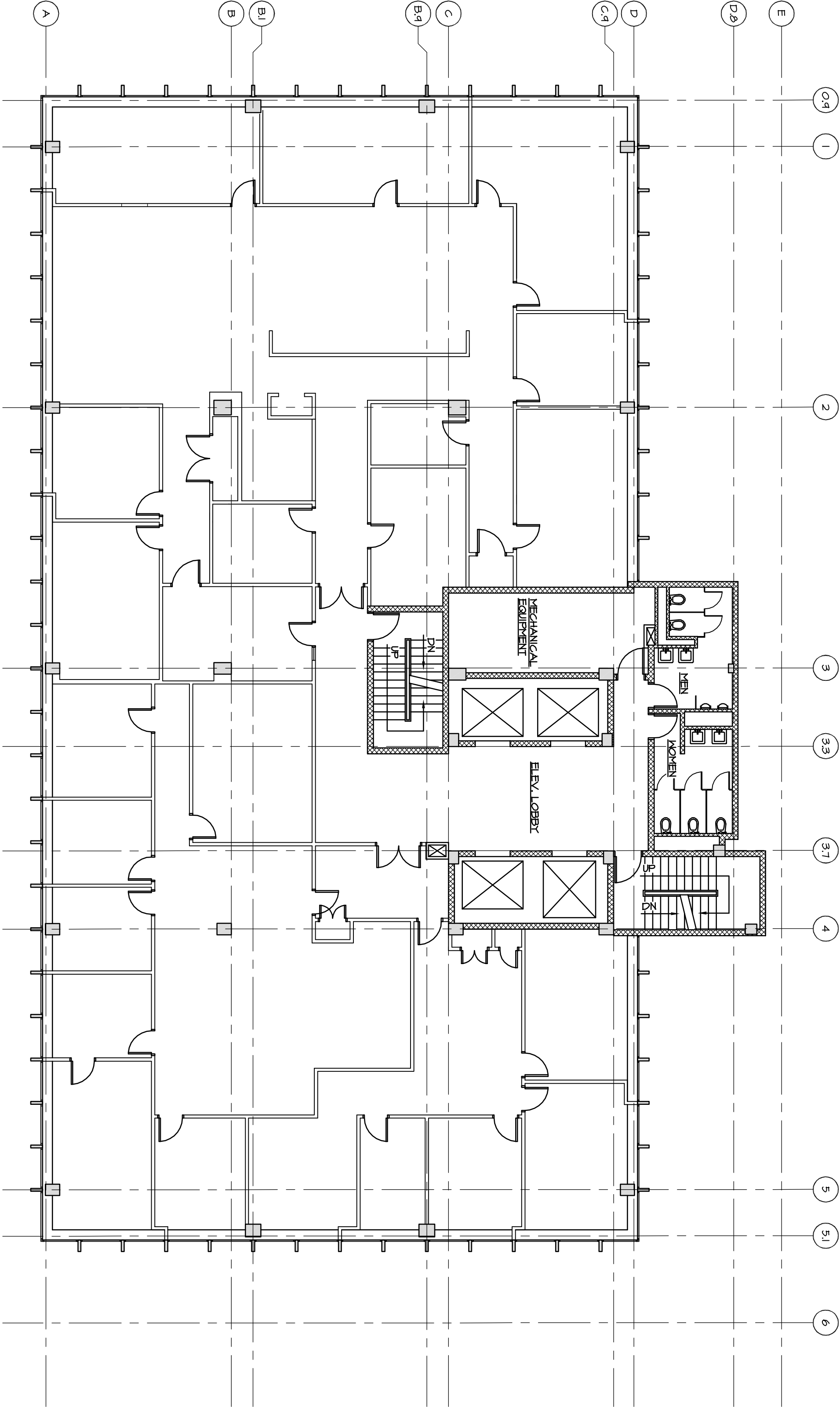
TENTH LEVEL FLOOR PLAN
